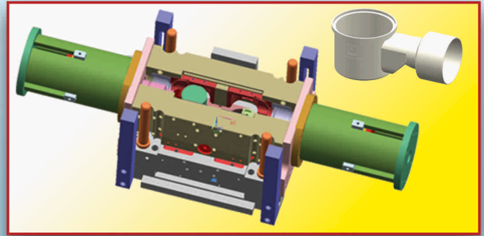
PVC Nahani Trap Mould
