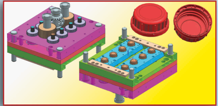
Break Cap Gear Mould
