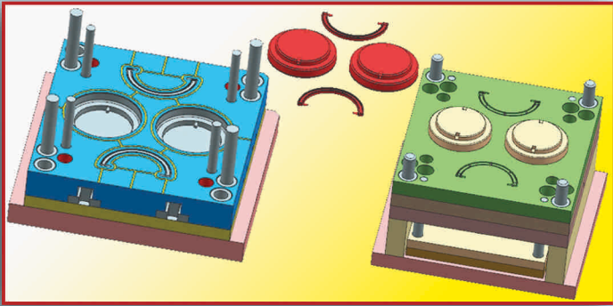
Handle Cap Mould
