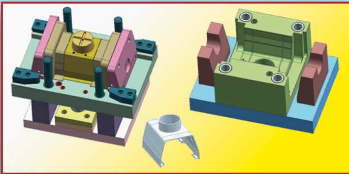
Rain Water Gutter Fitting Mould
