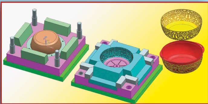
Double Moulded Bowl Mould
