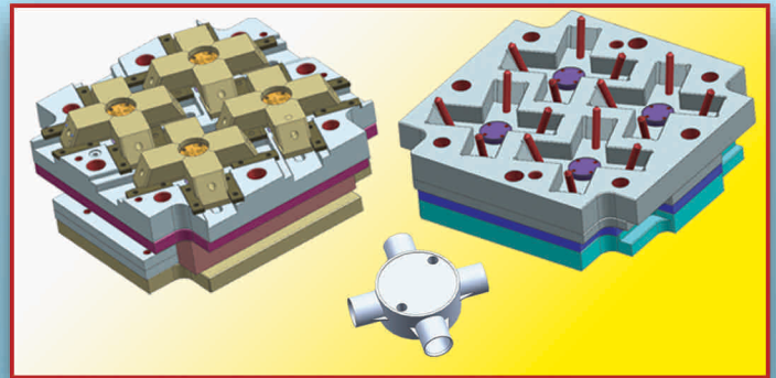
Junction Box Mould
